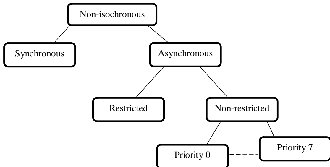
An overview of data transmission in FDDI
