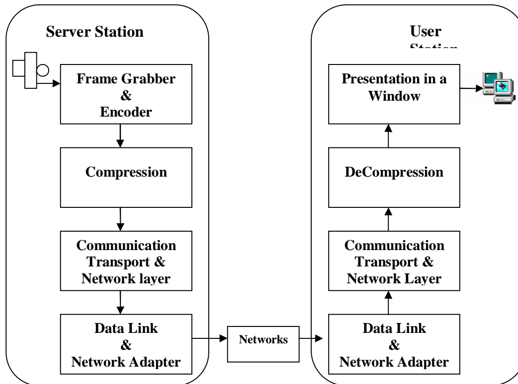
Components grouped for the purpose of video data transmission
