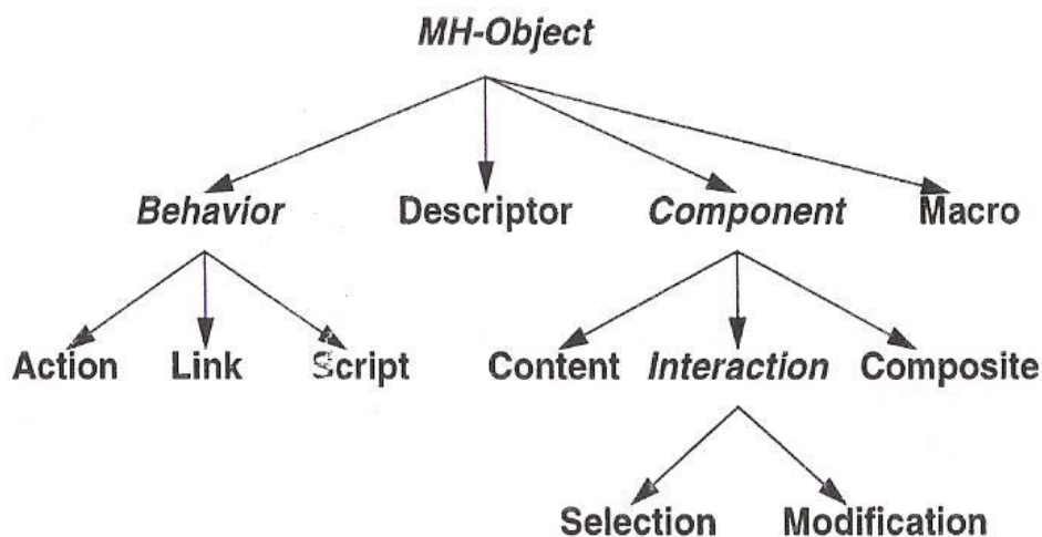
Class Hierarchy of MHEG Objects
