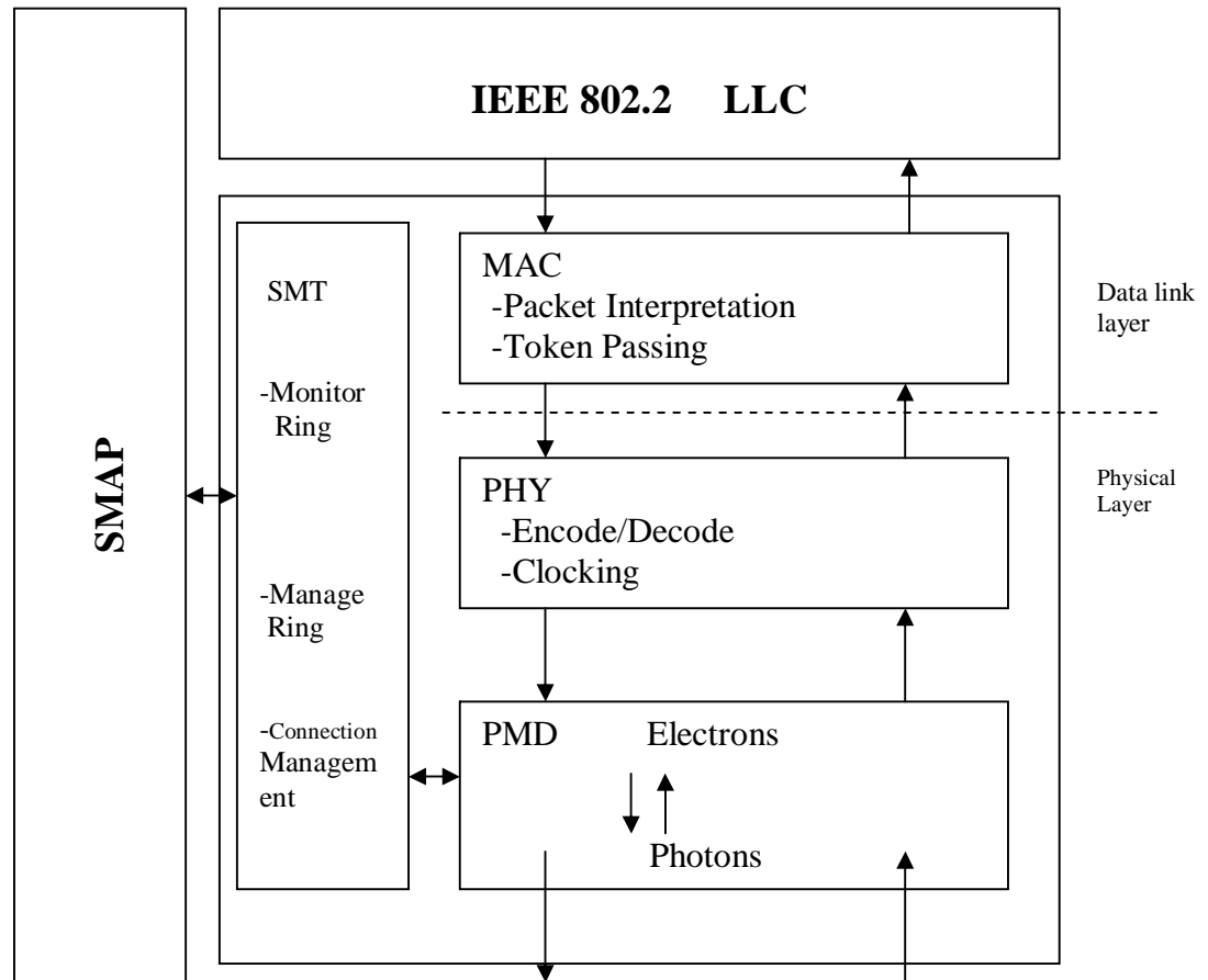
FDDI Reference model
