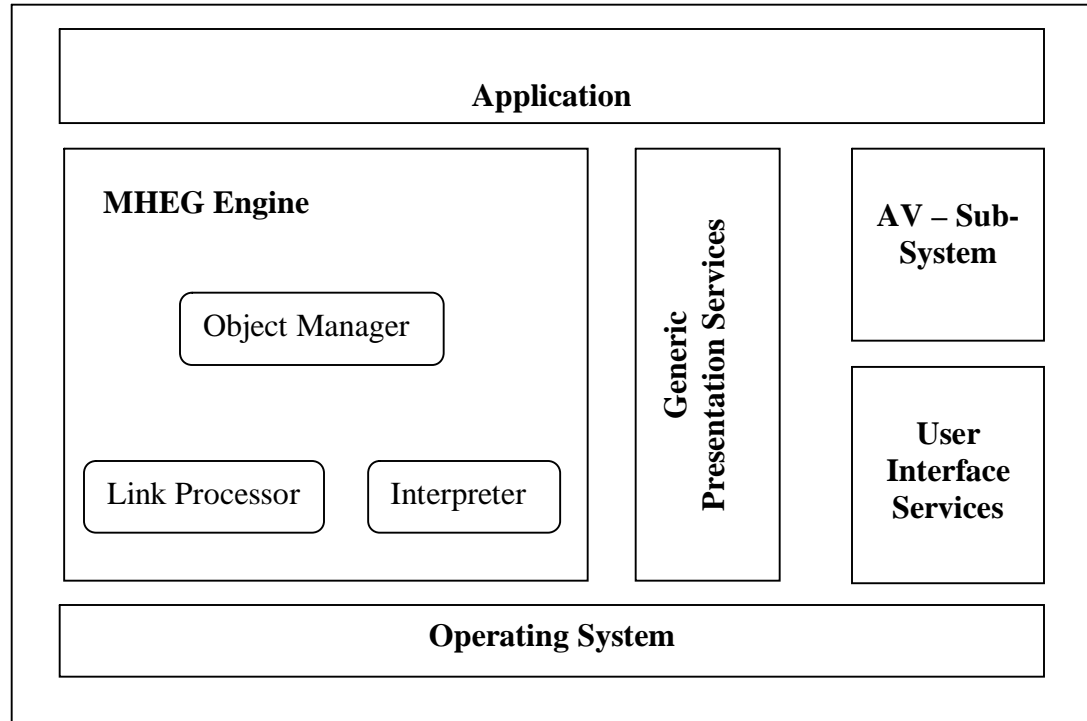
Architecture of an MHEG engine.
