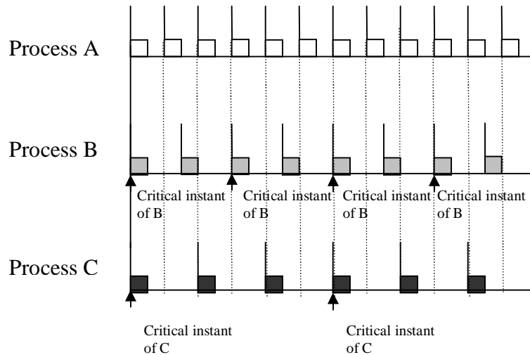
An example of critical instants
